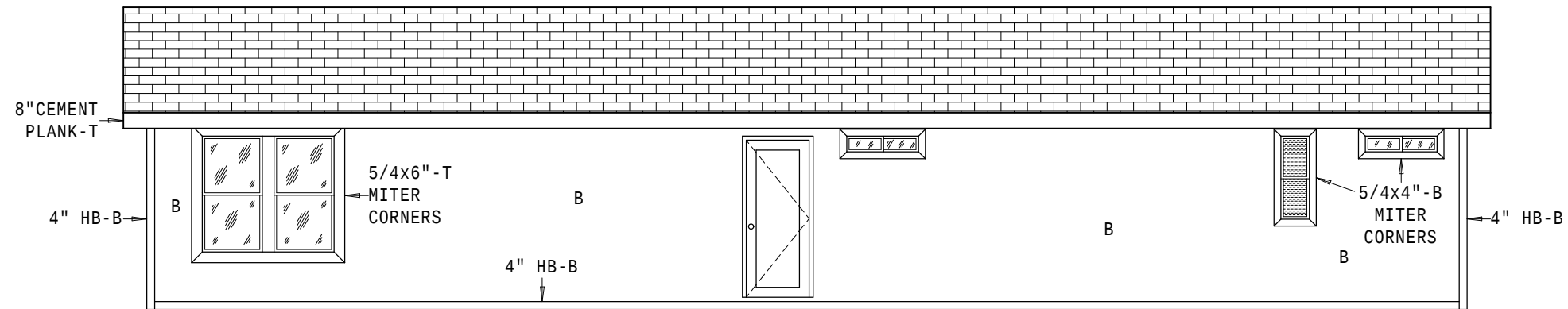
OFFDOOR SIDE ELEVATION
