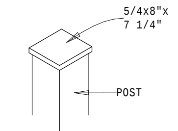
1/2 POST CAP DETAIL
