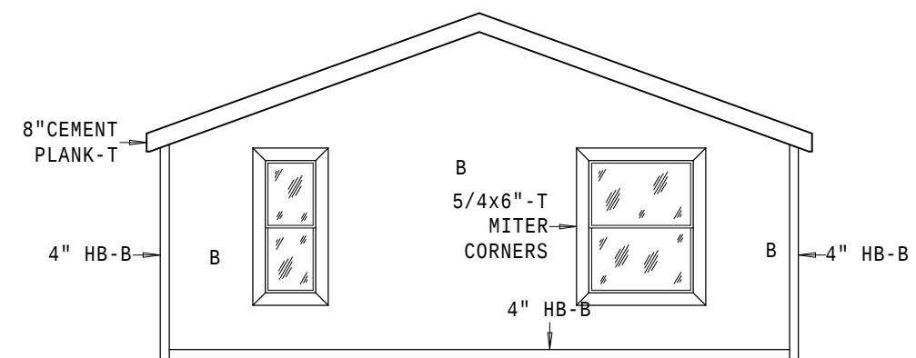
REAR ELEVATION
